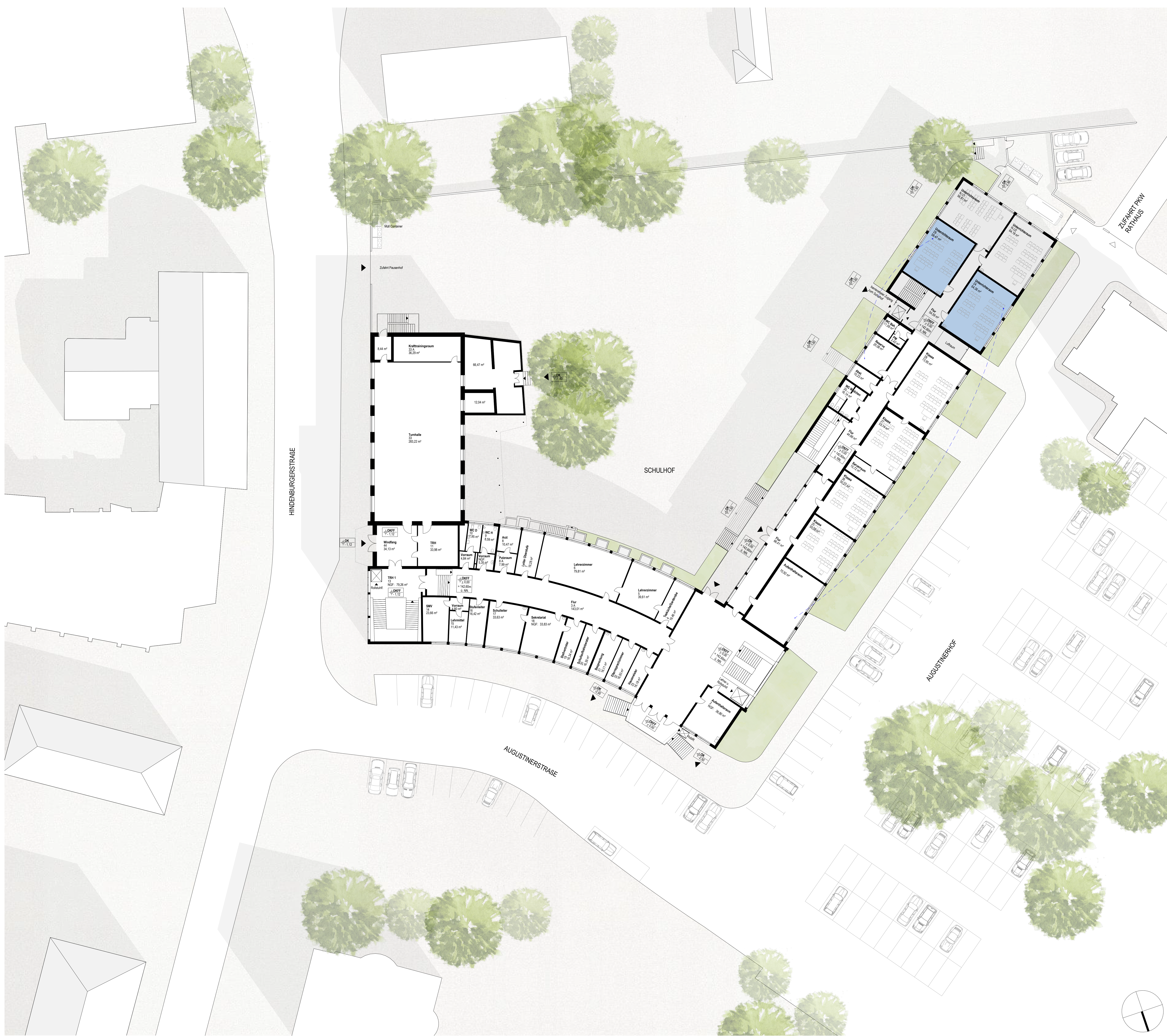
0. Erdgeschoss | M. 1:200
